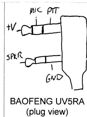
Figure 2: The plug and wiring that fit in the side jacks of the Baofeng. Note that the smaller connector is the earphone
